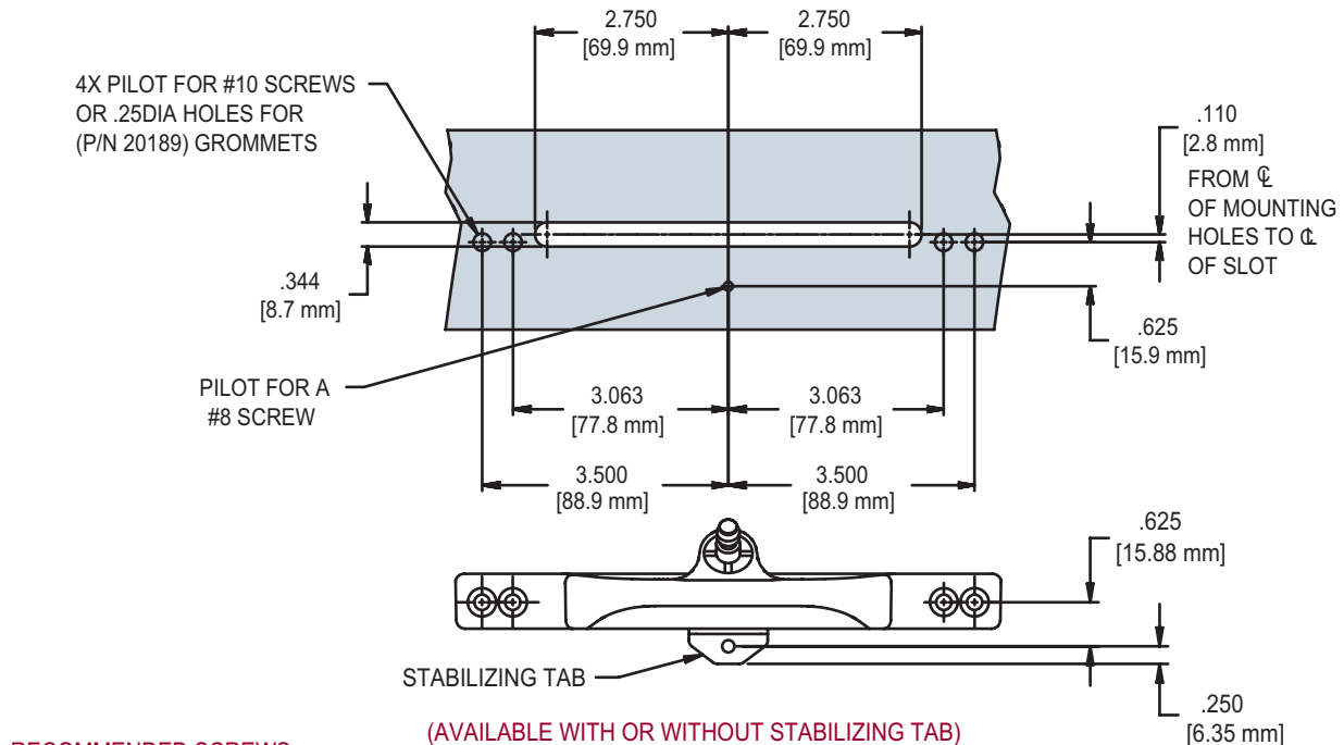
FIG. 2 FRONT MOUNT CUT OUT DETAILS
