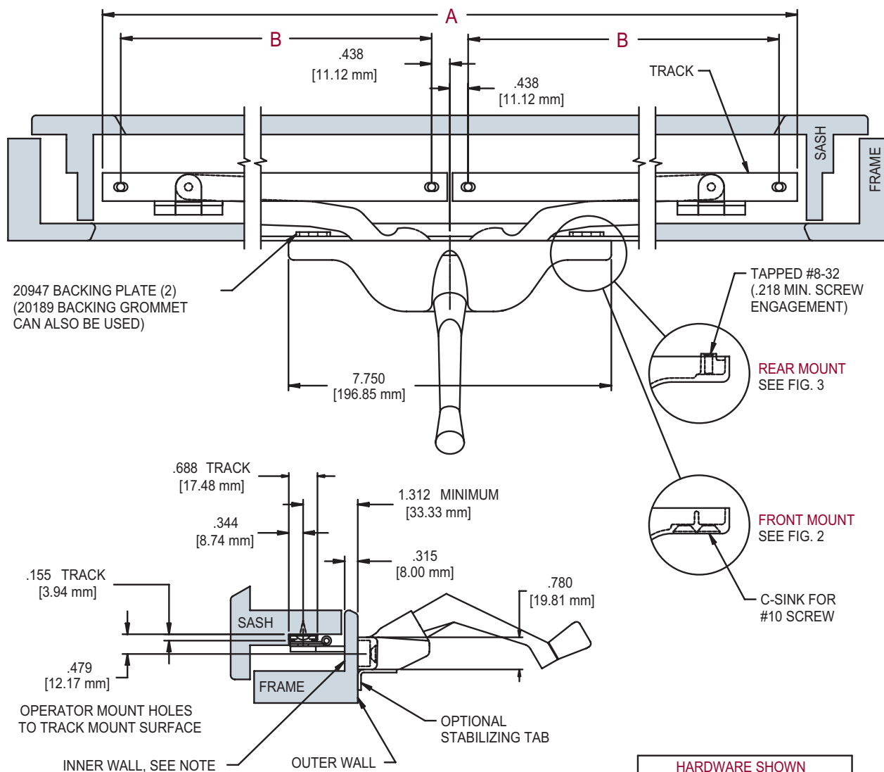
FIG. 1 APPLICATION OF 22 SERIES PIVOT SHOE OPERATOR
