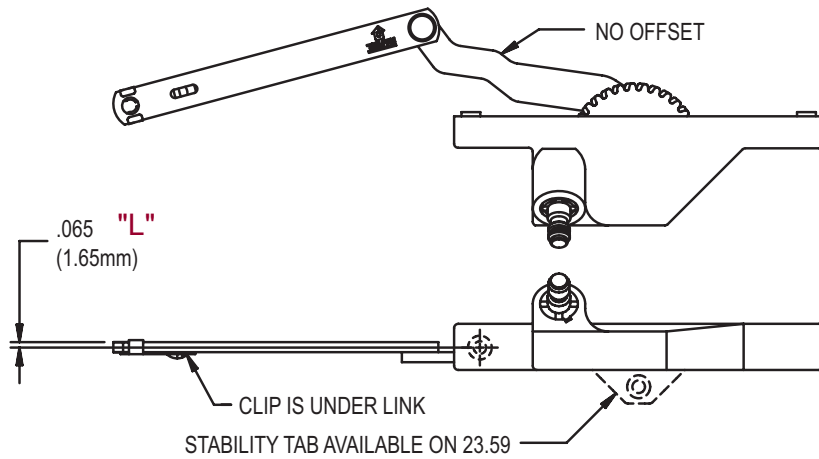
FIG. 3 23.46 and 23.59 DYAD OPERATOR (23.59 has stability tab)
