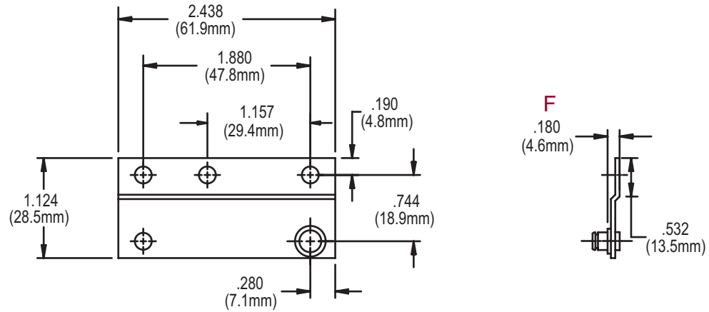
FIG. 11 STUD BRACKETS 10494.XX, 10495.XX
