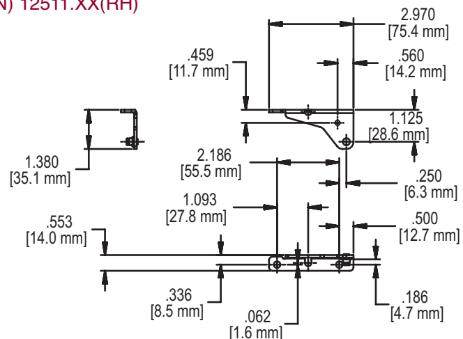
FIG. 6 STUD BRACKET 12510.XX(LH) (SHOWN) 12511.XX(RH)
